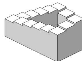
Penrose stairs
