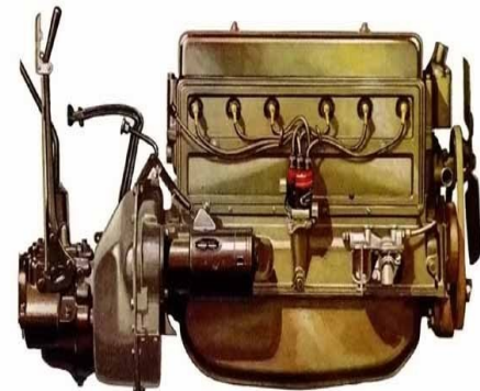
1929 CHEVROLET SIX-CYLINDER VALVE-IN-HEAD ENGINE
